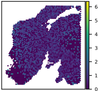
SNU24A DOCK9 expression Moran's I = 0.05
