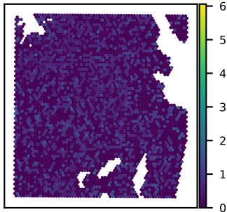
SNU51A BCS1L expression Moran's I = 0.02
