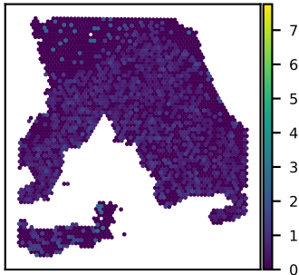
SNU18A CEP350 expression Moran's I = 0.06
