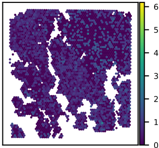
SNU16B EHBP1L1 expression Moran's I = 0.05
