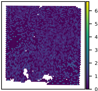
SNU43A C19orf12 expression Moran's I = 0.03
