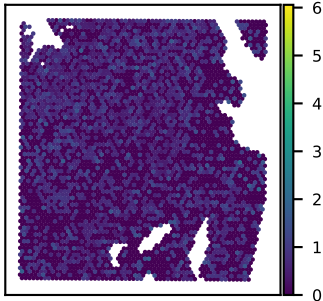
SNU51A TMED7 expression Moran's I = 0.02
