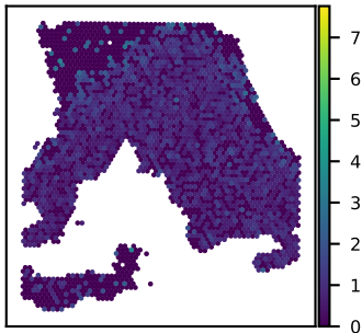
SNU18A FAAP100 expression Moran's I = 0.11
