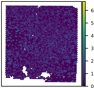
SNU43A METTL2A expression Moran's I = 0.02
