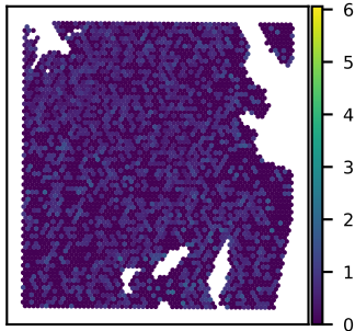
SNU51A PDPR expression Moran's I = 0.03
