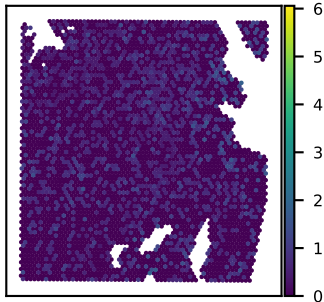
SNU51A KIF3B expression Moran's I = 0.02
