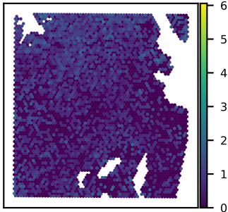
SNU51A CDK18 expression Moran's I = 0.16
