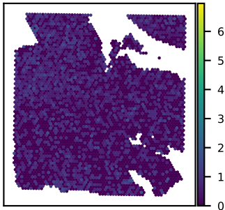
SNU24B C6orf136 expression Moran's I = 0.06
