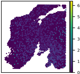
SNU24A TSPAN18 expression Moran's I = 0.10
