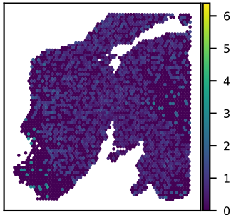
SNU24A CPPED1 expression Moran's I = 0.01
