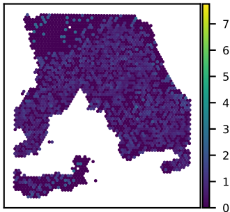
SNU18A TRNAU1AP expression Moran's I = 0.06
