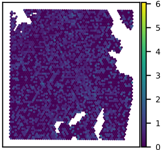
SNU51A DAAM1 expression Moran's I = 0.01
