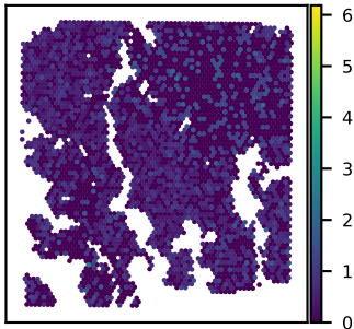
SNU16B SEMA4B expression Moran's I = 0.02
