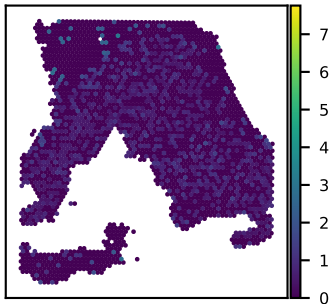
SNU18A DDX60L expression Moran's I = 0.03
