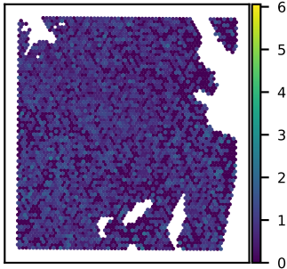
SNU51A TANC1 expression Moran's I = 0.04
