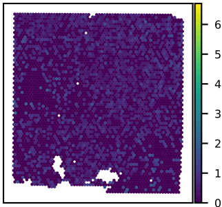
SNU43A PRMT3 expression Moran's I = 0.04
