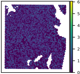
SNU51A IGBP1 expression Moran's I = 0.02
