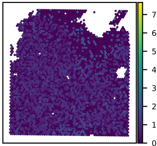
SNU21B TMEM150A expression Moran's I = 0.05
