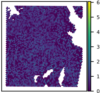
SNU51A TRIM13 expression Moran's I = 0.04
