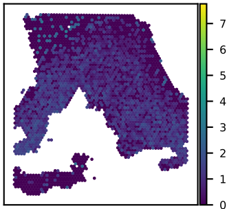
SNU18A BCL2A1 expression Moran's I = 0.26
