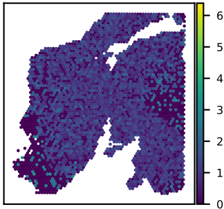
SNU24A GPBP1L1 expression Moran's I = 0.07
