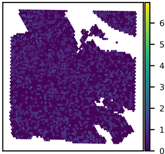
SNU24B ANKRD50 expression Moran's I = 0.01
