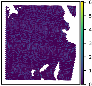
SNU51A PNPLA4 expression Moran's I = 0.02
