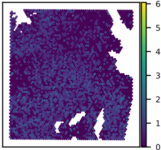
SNU51A HIST1H2AK expression Moran's I = 0.14
