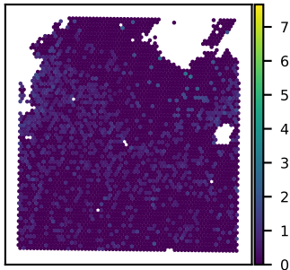
SNU21B PCDHB14 expression Moran's I = 0.11
