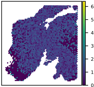
SNU24A C6orf89 expression Moran's I = 0.14
