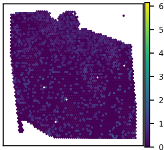
SNU27A SCFD2 expression Moran's I = 0.04
