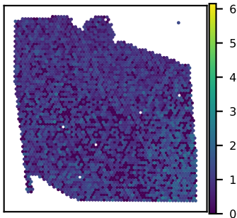
SNU27A PTPRF expression Moran's I = 0.04
