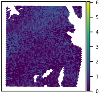
SNU51A PLXDC2 expression Moran's I = 0.22
