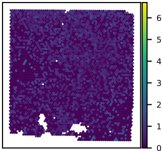
SNU43A BLVRA expression Moran's I = 0.05
