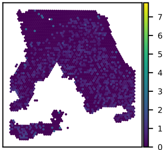
SNU18A NOS1AP expression Moran's I = 0.07
