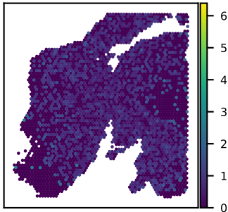
SNU24A TMEM250 expression Moran's I = 0.06
