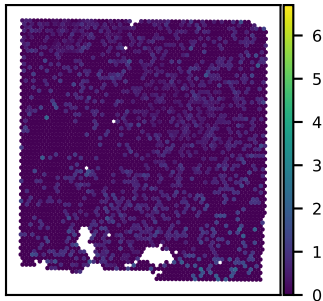
SNU43A SH3PXD2A expression Moran's I = 0.03
