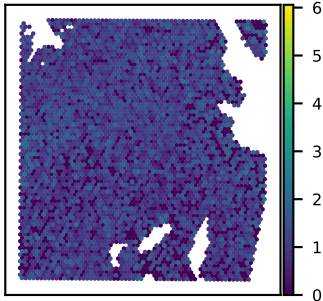
SNU51A PYURF expression Moran's I = 0.05
