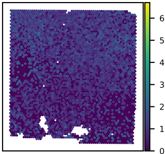
SNU43A GGT5 expression Moran's I = 0.15
