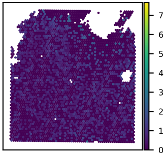
SNU21B SLC26A6 expression Moran's I = 0.03
