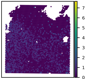
SNU21B TMEM178A expression Moran's I = 0.20
