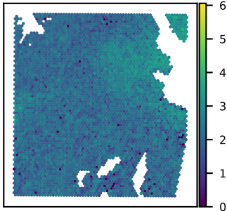
SNU51A CALM3 expression Moran's I = 0.35
