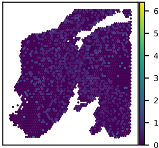
SNU24A MAP2K6 expression Moran's I = 0.04
