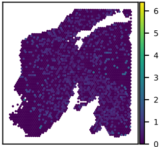
SNU24A FHOD3 expression Moran's I = 0.03
