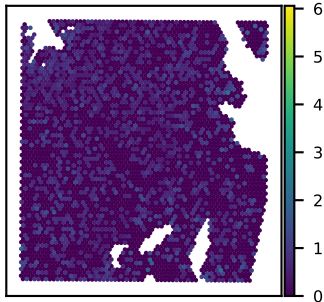
SNU51A TTC39C expression Moran's I = 0.04
