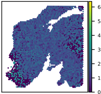
SNU24A CHMP2A expression Moran's I = 0.10
