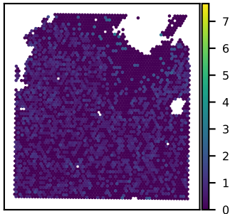
SNU21B NAA25 expression Moran's I = 0.05
