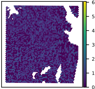
SNU51A TMEM101 expression Moran's I = 0.02
