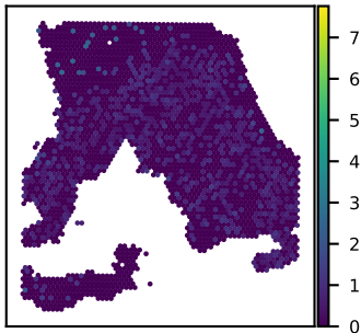
SNU18A ATP11C expression Moran's I = 0.04
