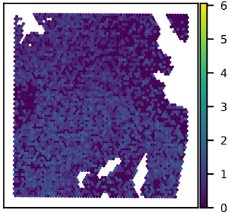
SNU51A CDCA7L expression Moran's I = 0.16
